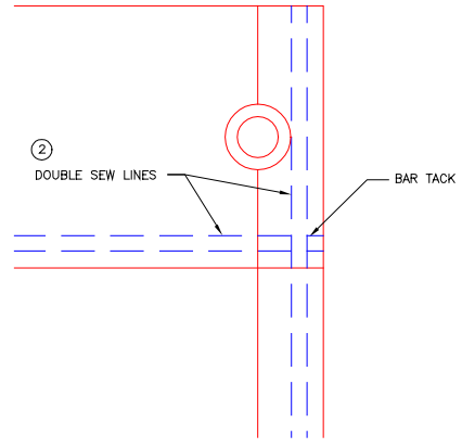
CORNER SEW DETAIL (BACK SIDE SHOWN) SCALE: 1/1
